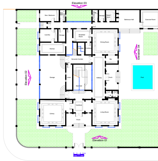
First Floor Plan A = 539,04 m 2
