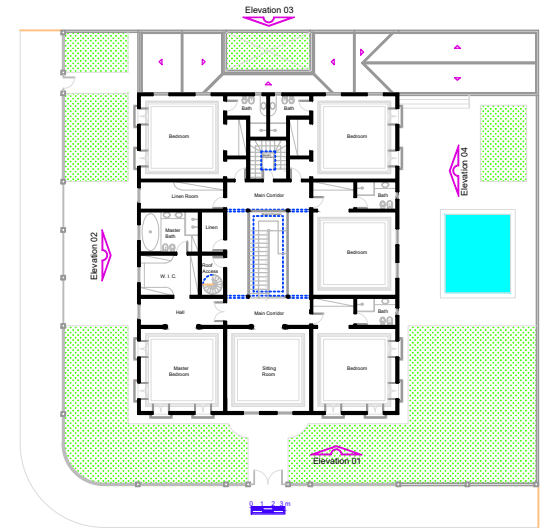
Second Floor Plan A = 413,73 m 2
